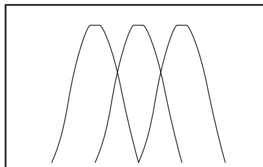
Figure 1.2. A measurement quality one-third octave filter
