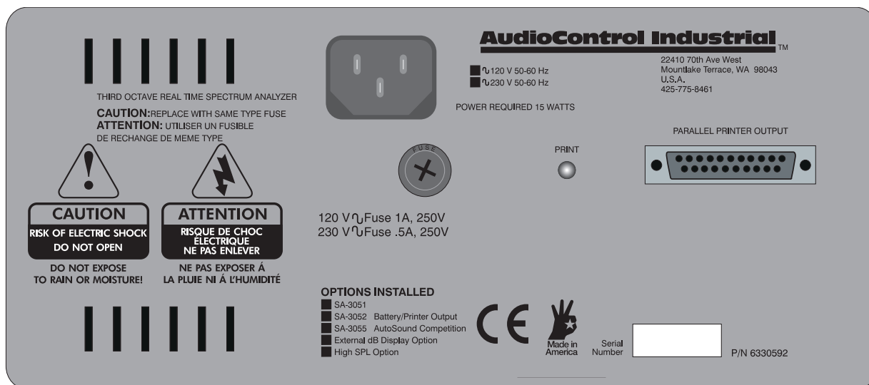
Figure 2.2. SA-3052A Rear Panel
