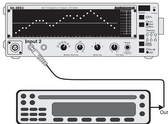
Figure 5.1. Checking a signal source
